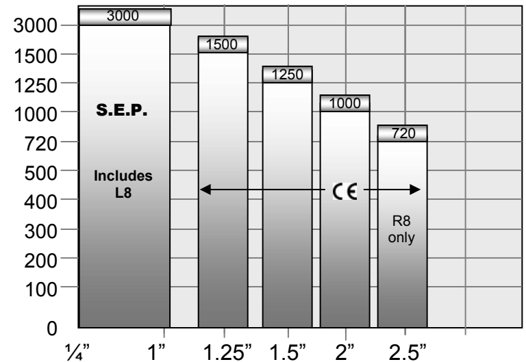
R8 & B8 Ratings According to CE/PED Cat. 1/Gp.2
