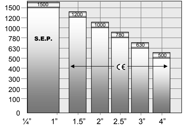
R8 & B8 Ratings According to CE/PED Cat. 1/Gp.2
