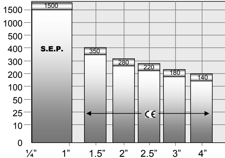
R8 & B8 Ratings According to CE/PED Cat. 1/Gp.1
